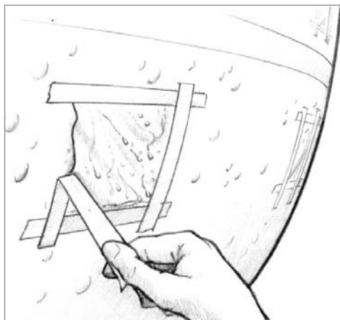
Figure 3-2 A piece of plastic taped to a wet hull will show condensation on the inside of the plastic.
