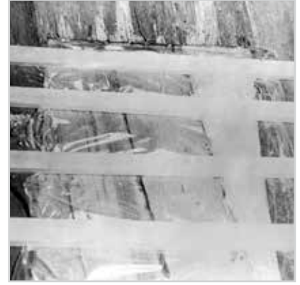
Figure 5-17 Cover the stringers with plastic to prevent bonding. (View from inside of hull).
