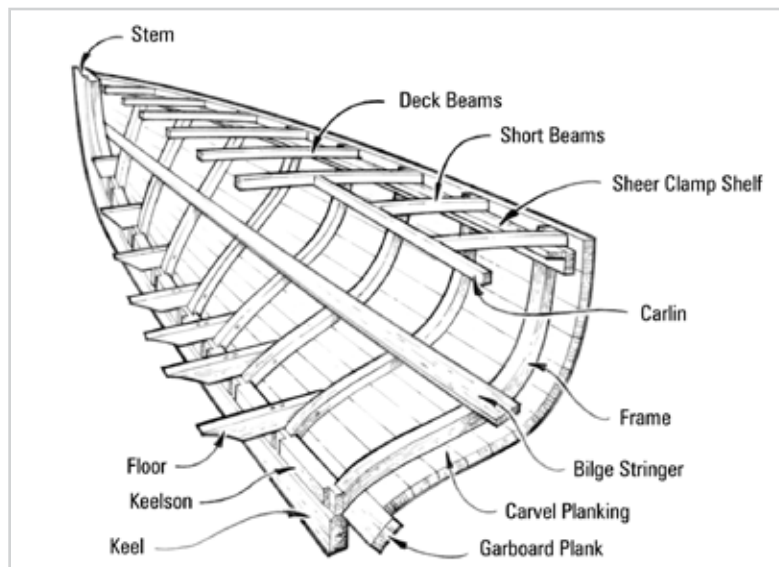
Figure 2-1 Typical structural framework.
