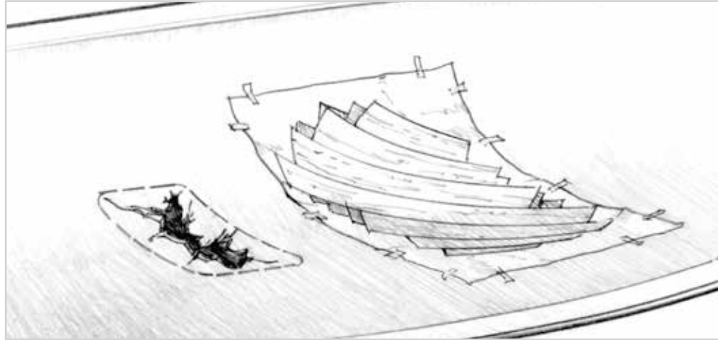
Figure 5-20 Laminate a replacement panel using the surface next to the damaged area as a mold.
