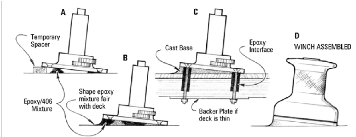
Figure 6-3 Hardware casting is an excellent method for installing a piece of hardware that is not flush to the deck such as a winch.
