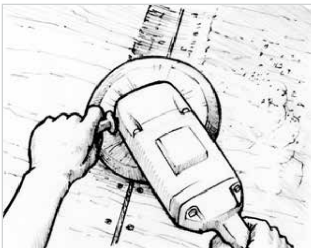
Figure 5-10 Sand a valley along the joint to allow for fiberglass tape.
