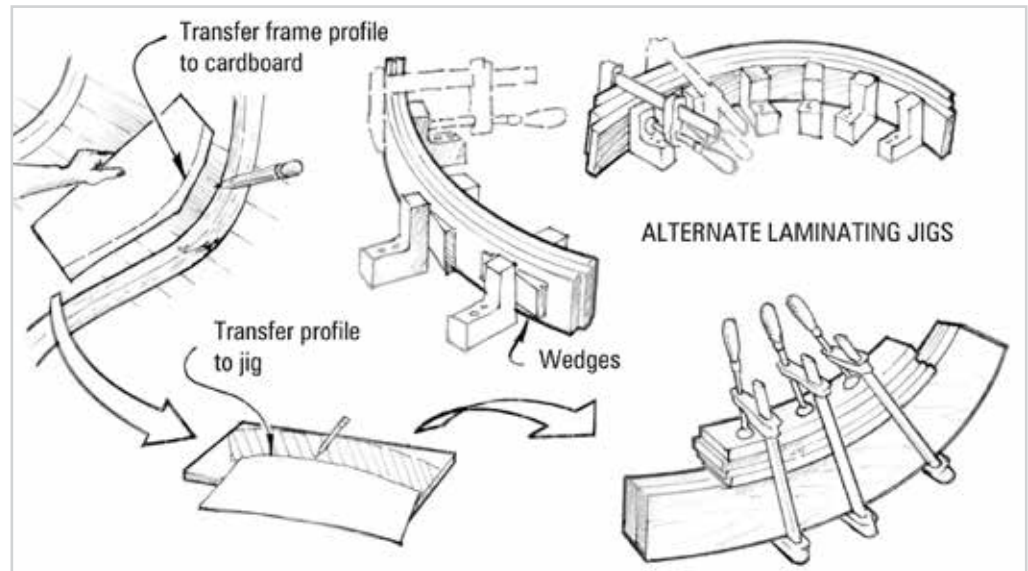
Figure 4-1 Transfer the desired frame shape to the jig.
