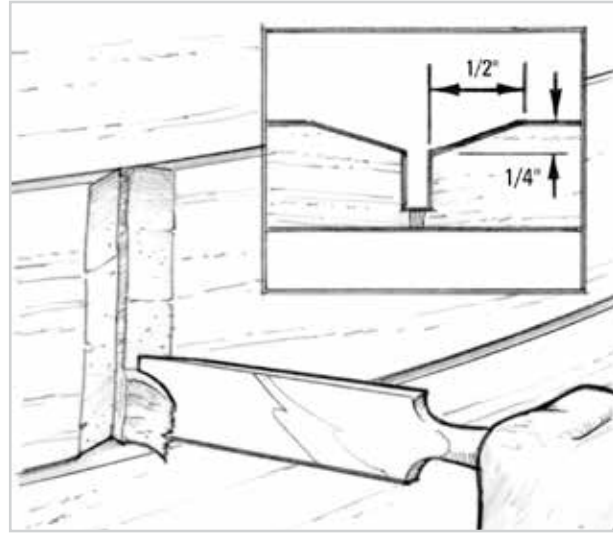
Figure 5-2 Cut a bevel on the end of each plank.
