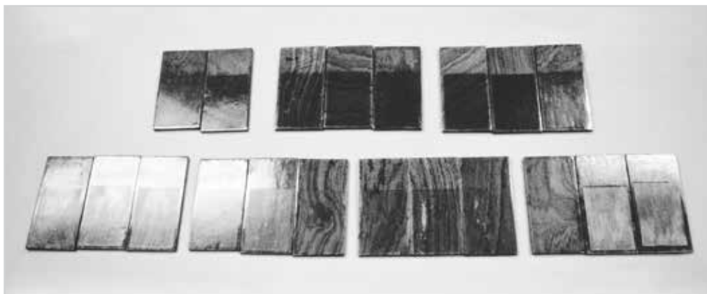
Figure 7-2 UV test samples after 3600 hours in weathering machine.
