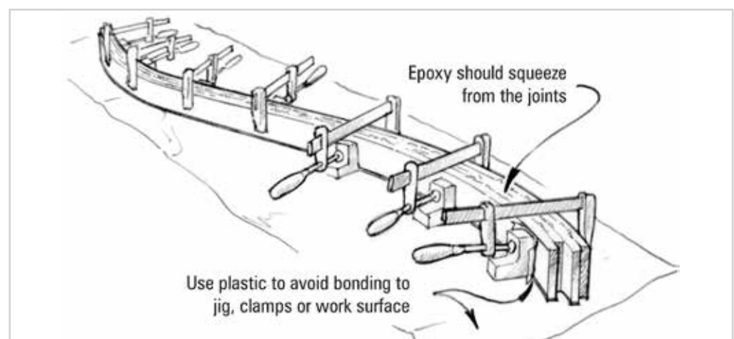
Figure 4-2 Clamp the appropriate number of coated strips into the jig. Trim the frame to size after the epoxy is fully cured.
