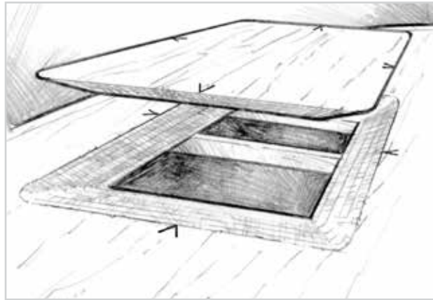
Figure 5-13 Clamp a new repair patch in position with staples or screws.
