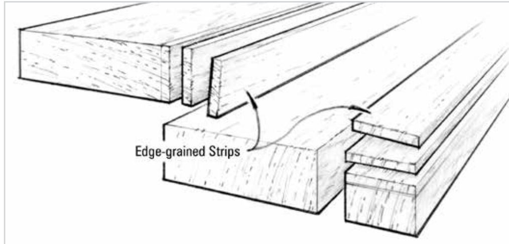
Figure 5-23 Thin edge-grained strips provide an even wearing, attractive and dimensionally stable deck.
