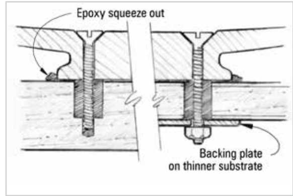
Figure 6-2 Tighten the fasteners until a small amount of epoxy squeezes from the joint.
