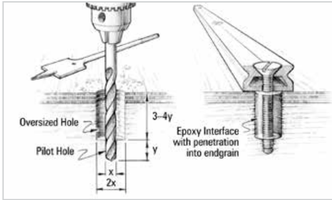
Figure 6-1 A normal sized pilot hole at the bottom of the oversized hole provides enough clamping pressure to hold the hardware in position until the epoxy cures.
