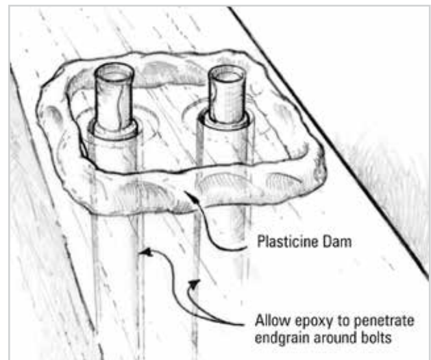
Figure 4-14 Build an epoxy reservoir around each keel bolt.
