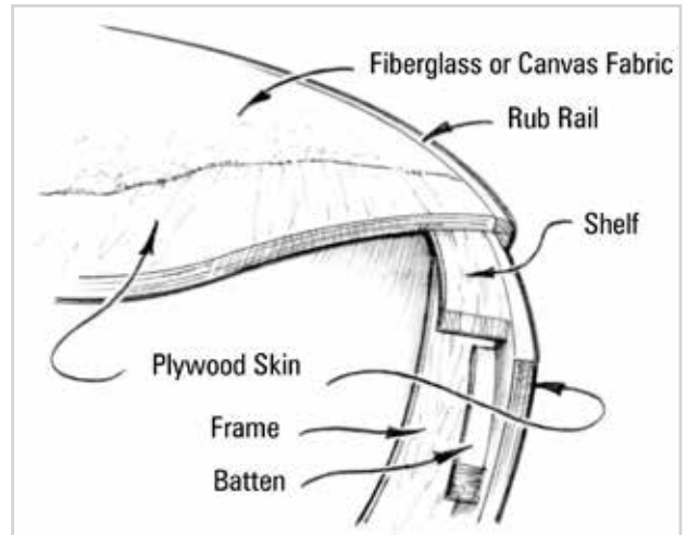
Figure 2-3 Typical plywood construction.
