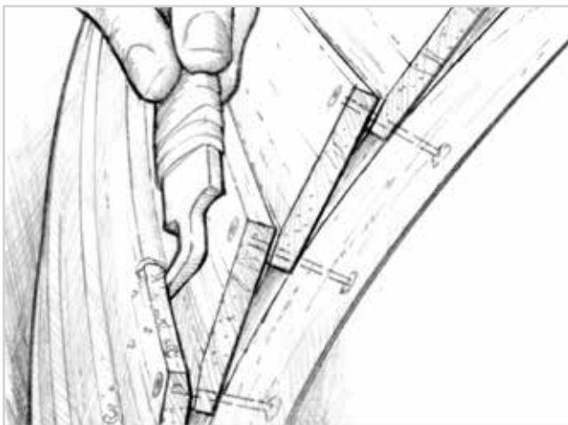
Figure 5-8 Clean out the seams with a scraper.
