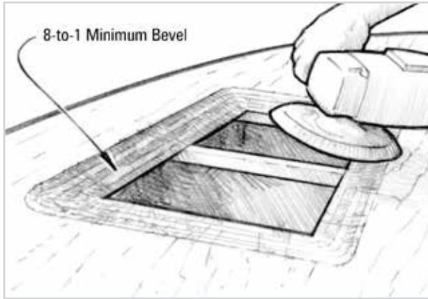
Figure 5-12 Cut out the damaged area and grind a minimum 8-to-1 bevel on all sides of the opening.
