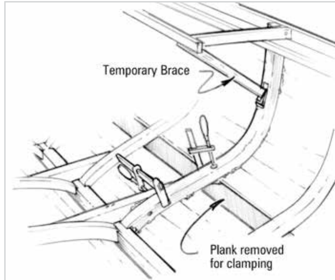
Figure 4-3 Install the new frame in the same position as the old frame. Braces or screws may be used to hold the frame until the epoxy cures.
